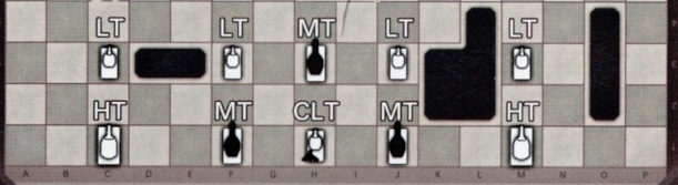
Starting positions of the white pieces
